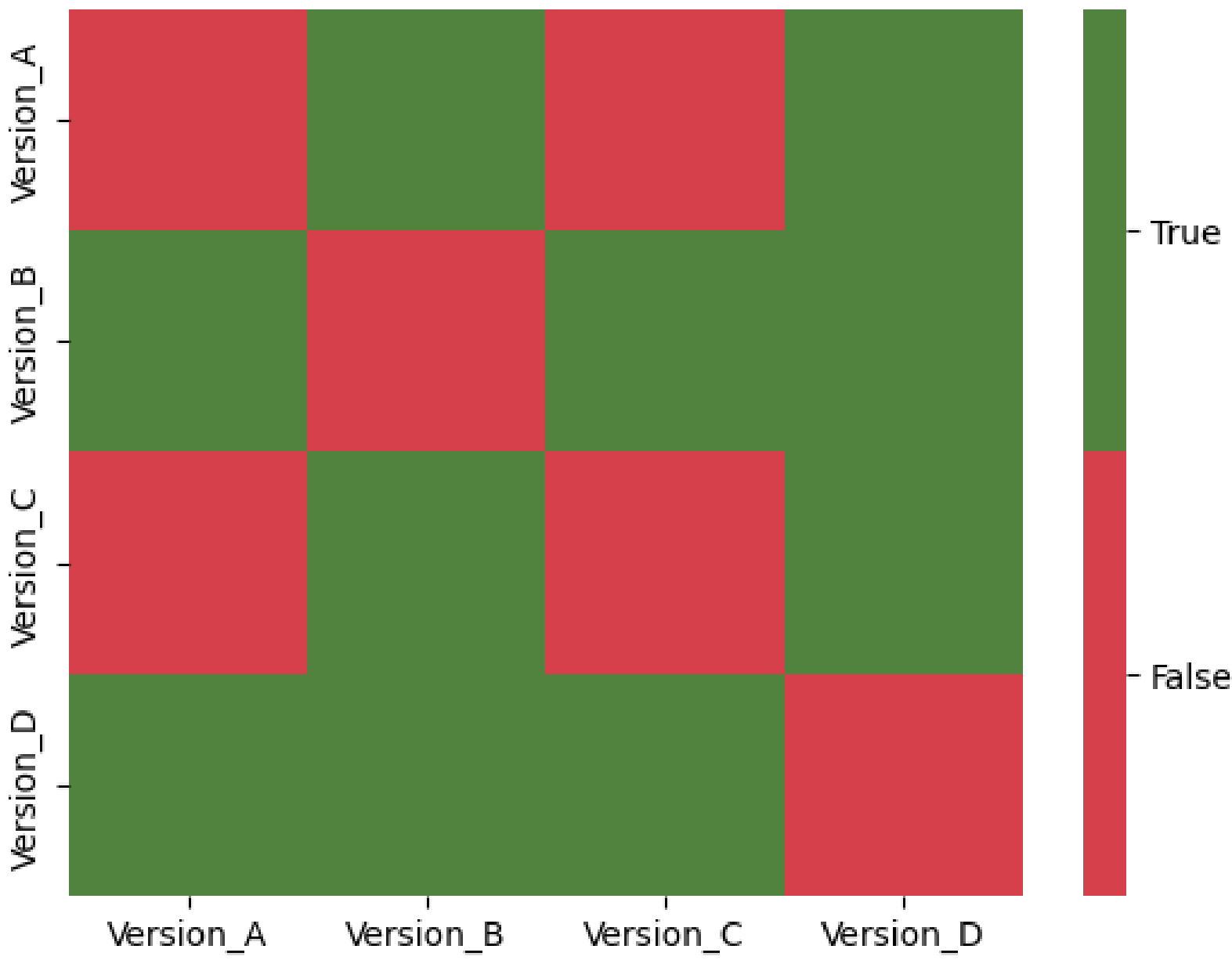
Statistical Significance in Pairwise Tests: True or False?
